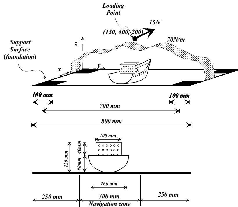
Figure 3. Geometrical overall requirements for the bridge models
