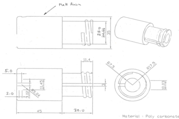
Figure 3 Final drawing of one component of the 'handle' in detailed design stage (exact reproduction of drawing )
