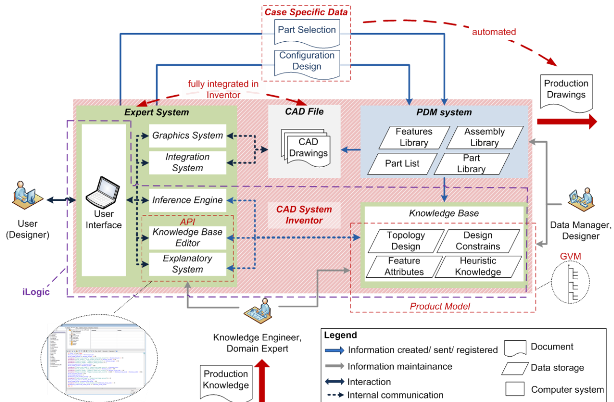
Figure 1 Integrated system architecture for automated precast design
