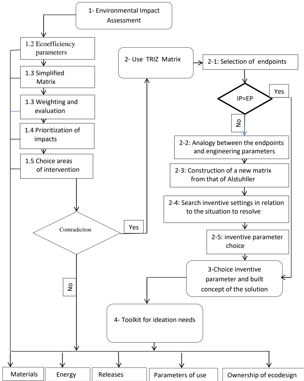
Figure 2. Initiative of the eco-innovating ECA-TRIZ process
