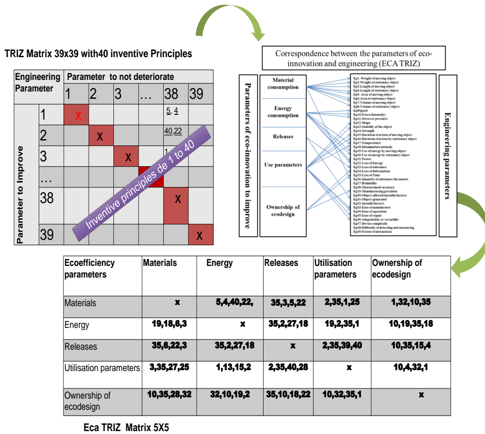
Figure 1. The approach to obtaining the ECA-TRIZ matrix
